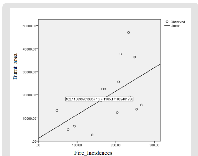
Figure 15: Correlation between fire incidence and burnt area at LTSMF
