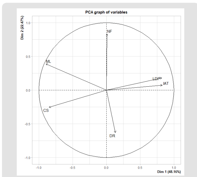
Figure 23: PCA showing causes of forest fire in Dhanusha district.
