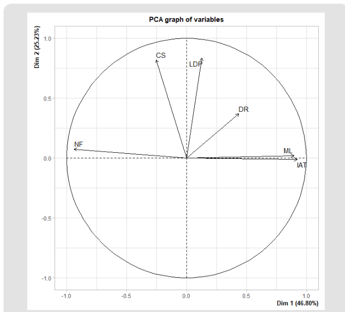
Figure 22: PCA showing causes of forest fire in Mahottari district.
