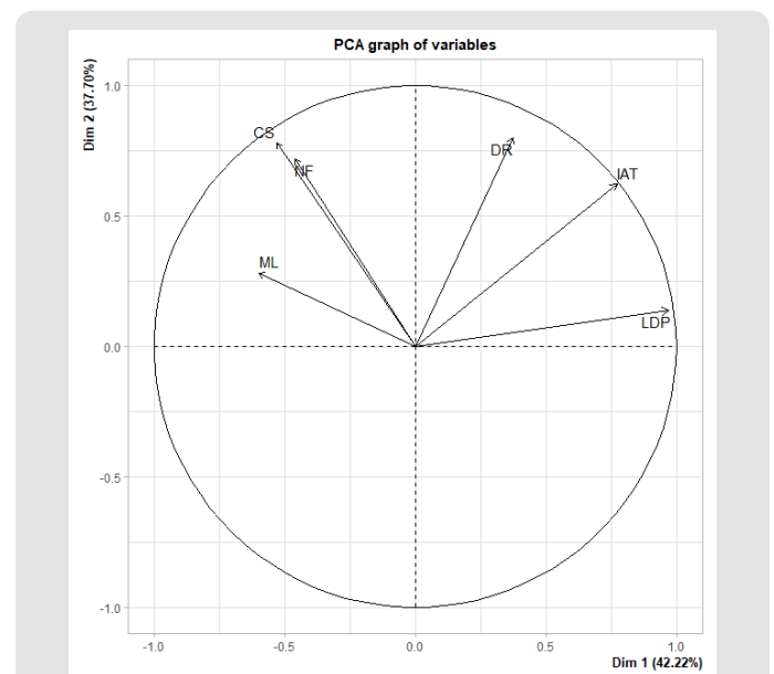
Figure 24: PCA showing causes of forest fire in Siraha district.
