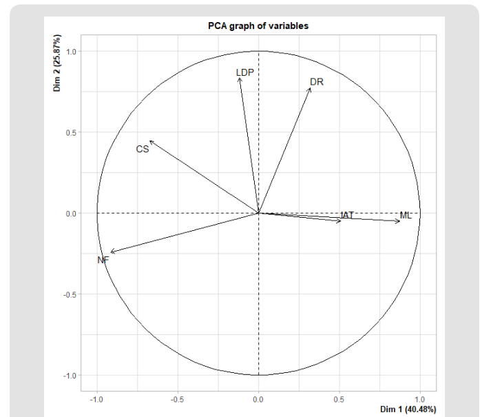
Figure 20: PCA showing causes of forest fire in Rautahat district
