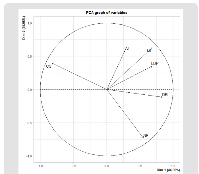
Figure 25: PCA showing causes of forest fire in Saptari district.
