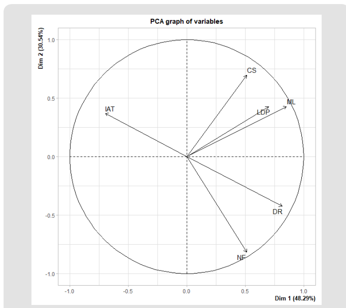
Figure 19: PCA showing causes of forest fire in Bara district
