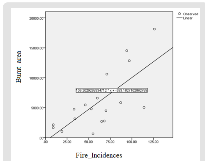
Figure 16: Correlation between fire incidence and burnt area at HSF.
